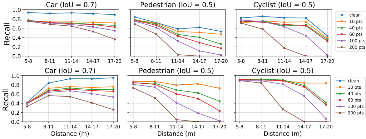
Fig. 2. Recall metrics by distance (in metres away from the LiDAR) for different IoU configurations of (top) PointRCNN and (bottom) Point-GNN.
