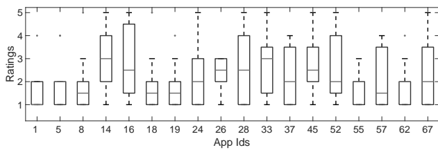
Figure 9: Apps for which the usual consensus is that they are not performing any text detection or recognition. The x-axis represents the app ids and the y-axis represents the ratings. Ratings are on a scale of 1 to 5, where 1 represents strong disagreement and 5 strong agreement. Note that all apps had been observed performing text detection.
